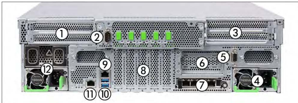
Figure 10: AU47 M7 (rear)
