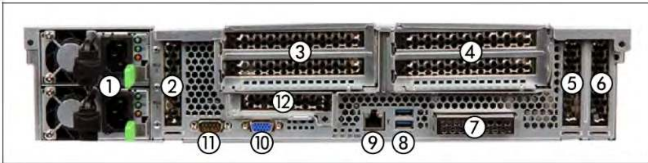
Figure 6: AU47 M5 - rear
