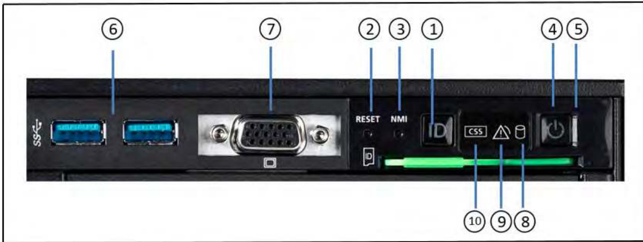
Figure 2: AU47 M5 (front) - Detailed view: operator control panel
