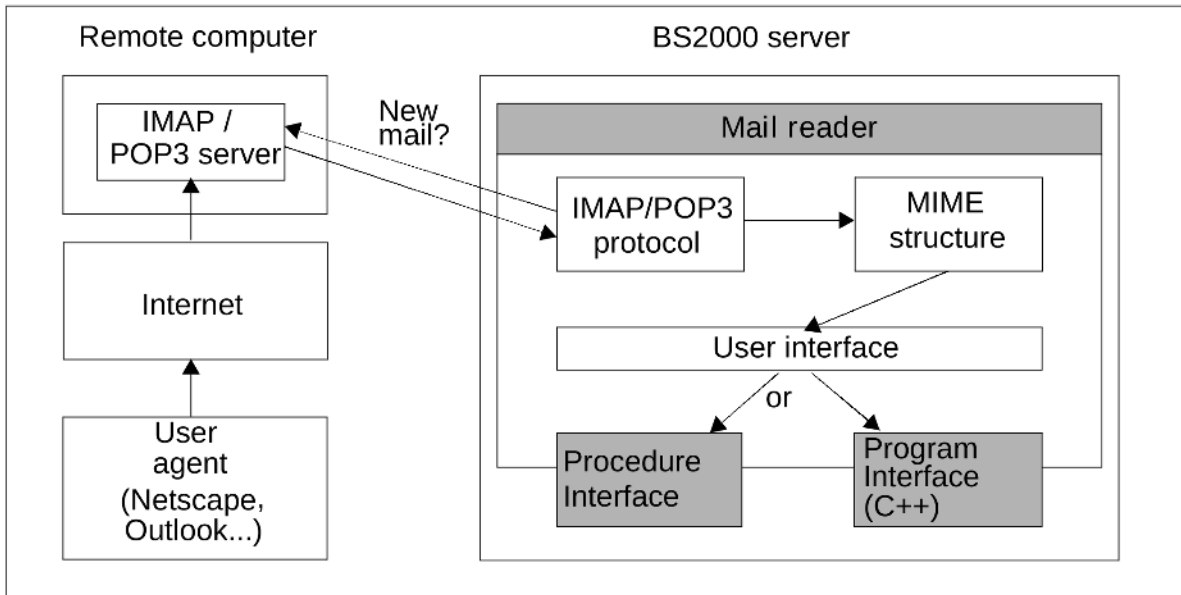
Figure 8: Mail reader in BS2000
