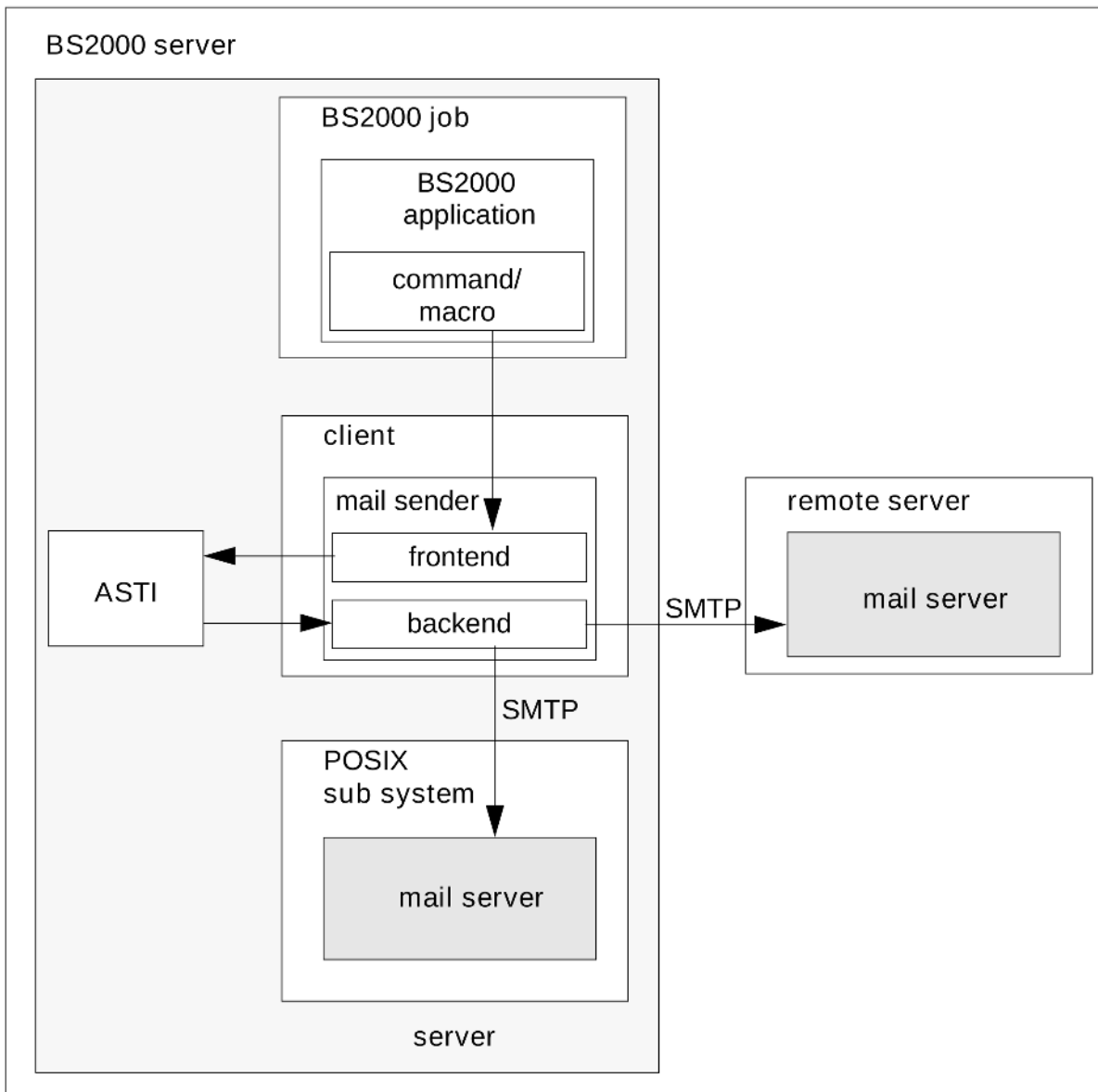
Figure 9: Mail sender in BS2000
