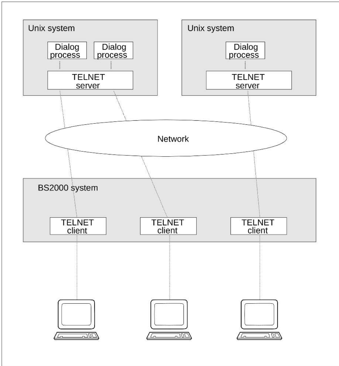
Figure 5: TELNET clients in BS2000
